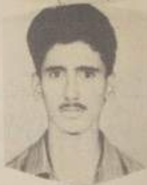
Nandakumar Physics
